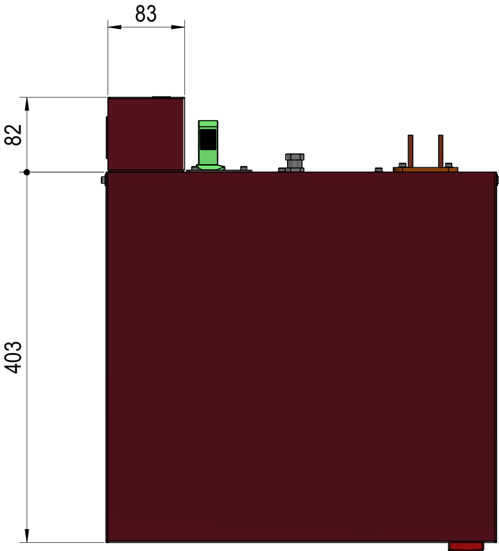
TOP VIEW
